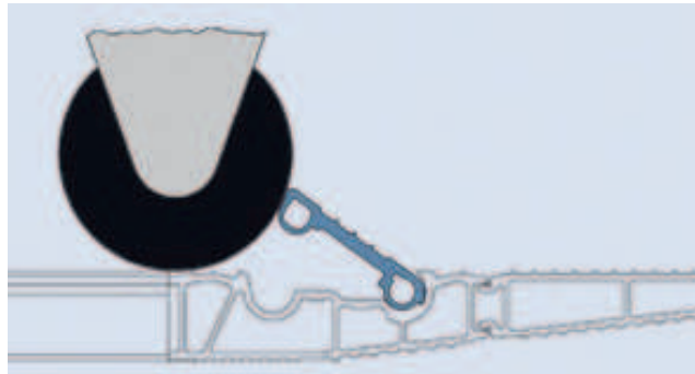
Trolley stop rd as a barrier for rollers with an opening angle of 43° for roller diameter up to 110 mm. Flap width: 850 mm with min. platform width of 2400 mm.
