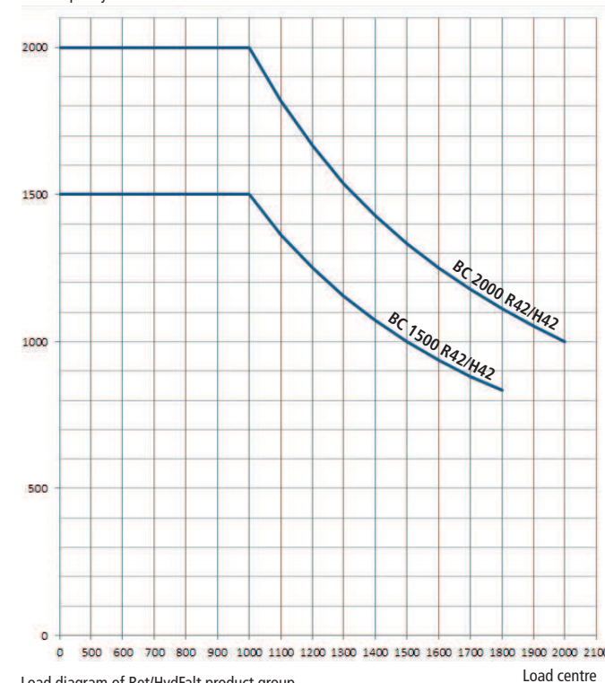
Load diagram of Ret/HydFalt product group
