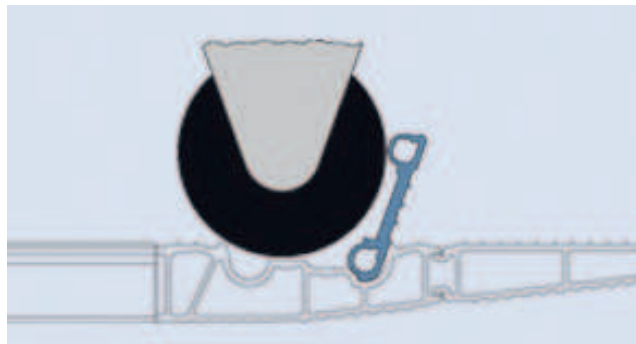
Trolley stop ad as a recess for rollers with an opening angle of 110° for roller diameter up to 200 mm. Flap width: 850 mm with min. platform width of 2400 mm.
